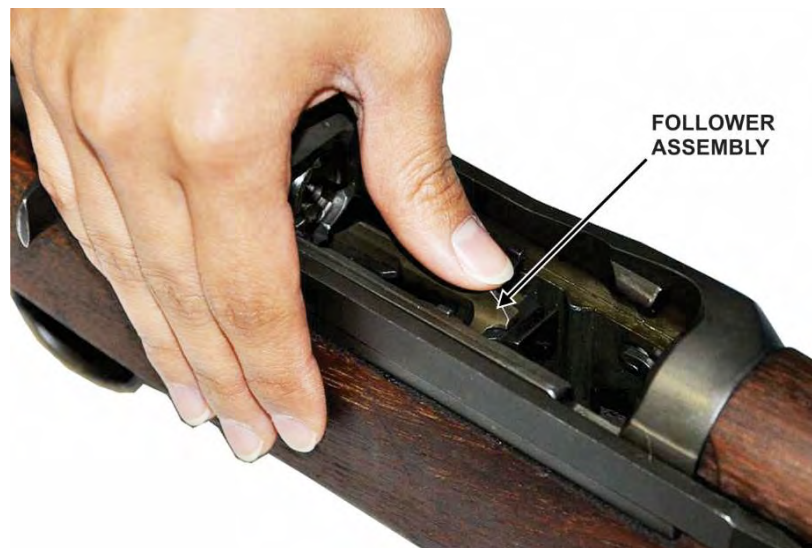
Figure 9. Depressing the follower assembly
