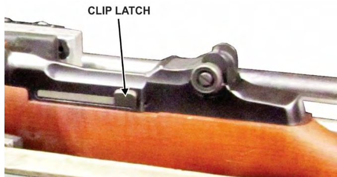
Figure 57. Clip latch
