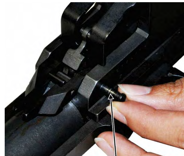
Figure 48. Follower arm engaged
